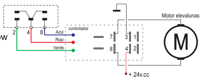
892010 Inverter for electric motor rotation (1 Amp)
